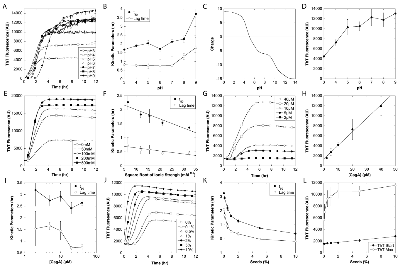
Figure 1. Effect of environmental conditions on the fibrillation of CsgA. (A, E, G, and J) Fibrillation of CsgA followed by ThT at various pH values (A), NaCl concentrations (E), protein concentrations (G), and CsgA fibril seed concentrations (J). The standard conditions for the fibrillations were 20 \mu M CsgA in 20 mM sodium phosphate (pH 7) without addition of NaCl or seeds. (B, F, I, and K) Effect of pH (B), ionic strength (F), protein concentration (I), and CsgA fibril seeds (concentrations in weight percentage) (K) on the kinetic parameters t_{50} and lag time. (C) Theoretical overall charge of mature CsgA as a function of pH calculated using CLC DNA Workbench version 5.7.1. (D and E) Effect of pH (C) and protein concentration (H) on the ThT maximum. (L) Effect of seeds on ThT start level and maximum.
