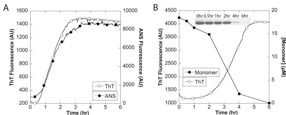
Figure 5. Fibrillation of CsgA followed by ANS fluorescence and SDS-PAGE. (A) Fibrillation of 20 \mu\text{M} CsgA followed by ThT and ANS fluorescence. (B) Fibrillation of 20 \mu\text{M} CsgA followed by ThT and SDS-PAGE. SDS-PAGE data were expressed as the CsgA monomer concentration calculated from the CsgA monomer band intensity using the ImageJ gel analysis tool ( http://rsbweb.nih.gov/ij/ ).
