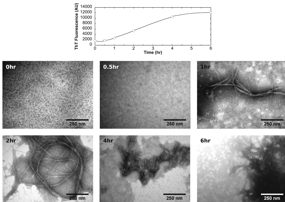
Figure 4. Fibrillation of CsgA followed by TEM. Samples were collected at various time points during the fibrillation of 40 \mu\text{M} CsgA at pH 7 and examined by TEM. The fibrillation curve measured by ThT is shown at the top, with circles corresponding to the time points shown in the bottom panels.
